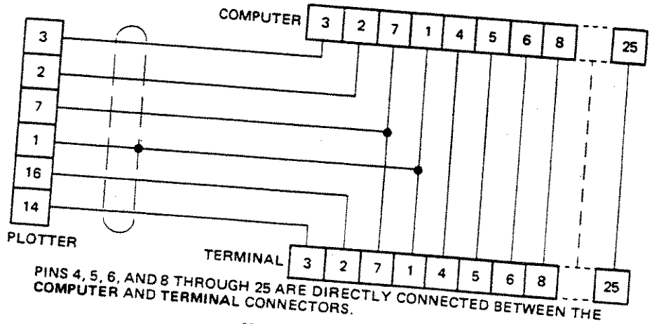
Y-cable Schematic
